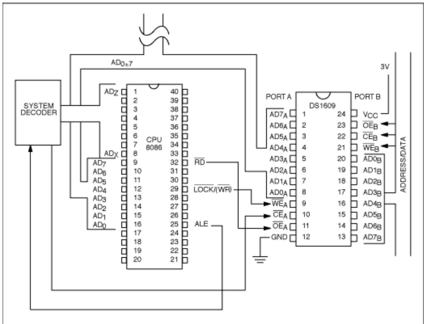
Figure 1. DS1609 Dual Port Interface to Intel 8086 Microprocessor
