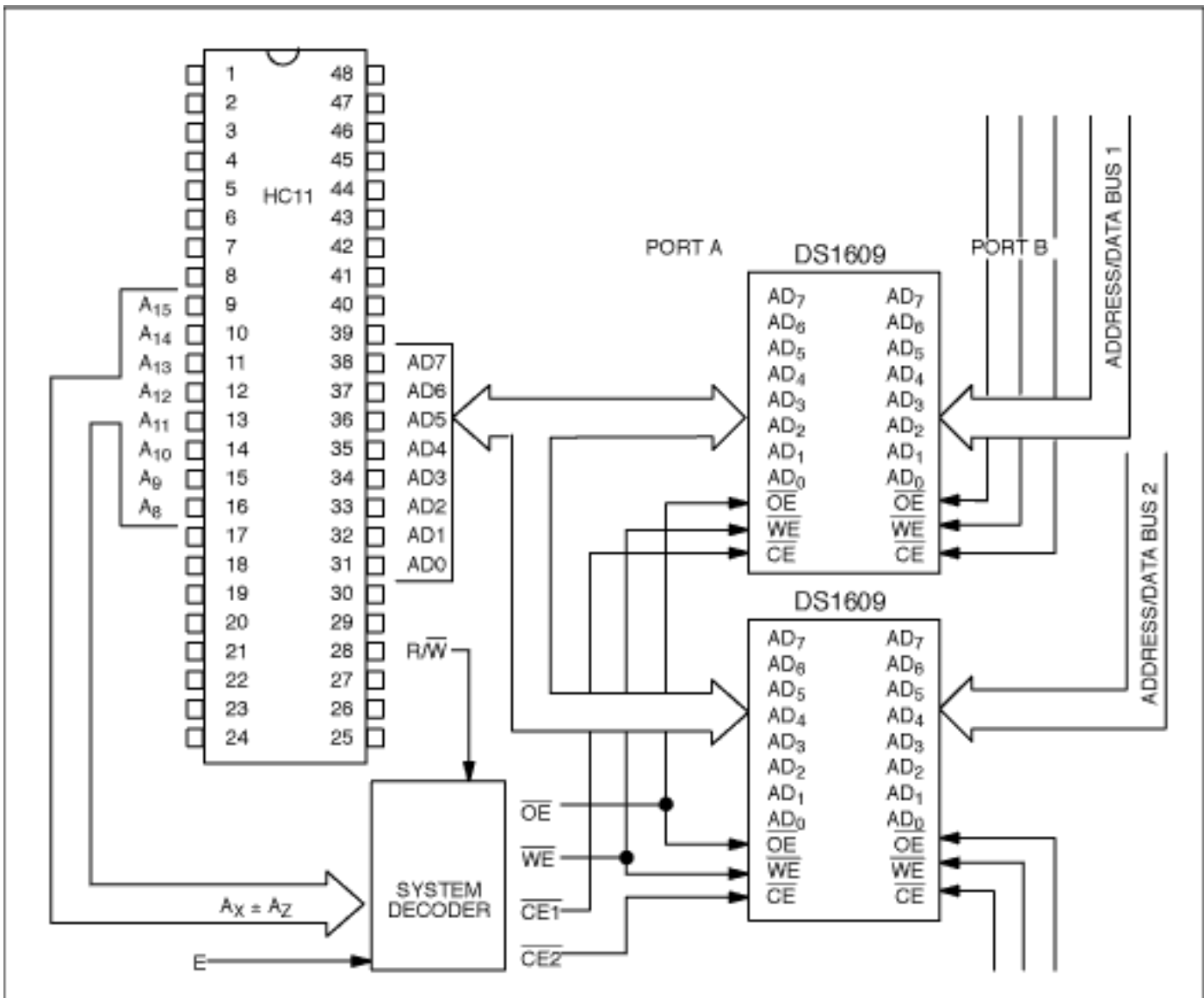
Figure 4. Motorola HC11 Expanded Mode Multiple DS1609's
