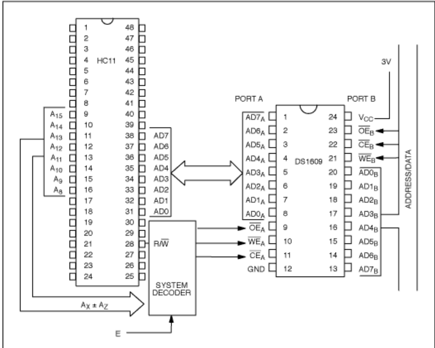
Figure 2. Motorola HC11 Expanded Mode
