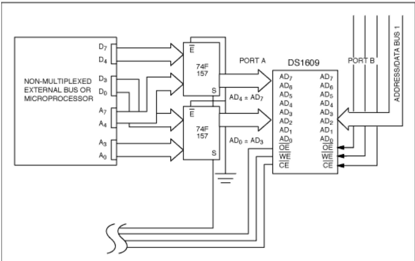
Figure 5. Sample Implementation; Non-Multiplexed Bus
